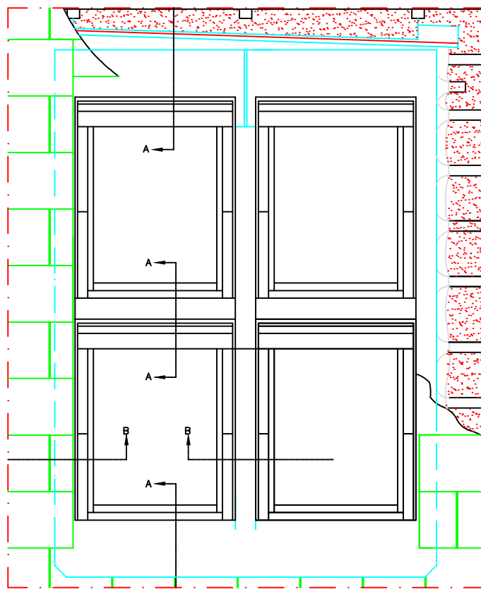
TYPICAL ELEVATION
